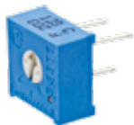
1 VOLTA - RE F. 3386F 23.36.003 100R..... 23.36.004 200R..... 23.36.006 1 K..... 23.36.007 2 K..... 23.36.008 5 K..... 23.36.009 10 K..... 23.36.010 20 K..... 23.36.011 50 K..... 23.36.012 100 K..... 23.36.013 200 K..... 23.36.014 500 K..... 23.36.015 1 M.....
